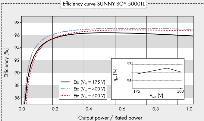
Efficiency curve SUNNY BOY 5000TL
